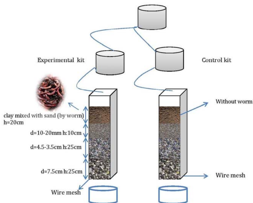
Figure 1) A scheme of the vermifiltration kits
